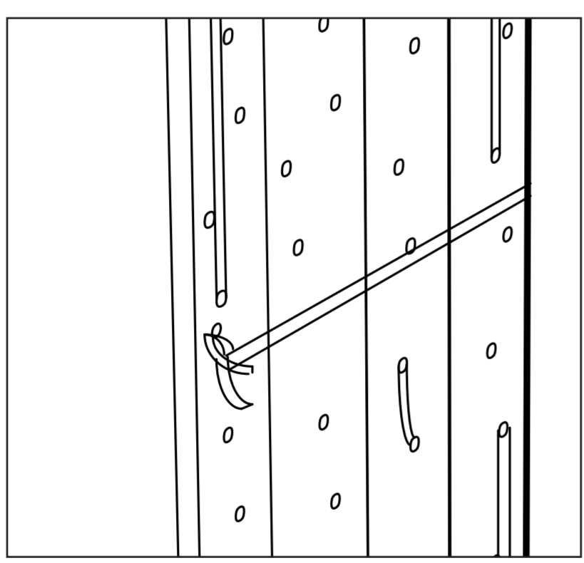
Detail B
