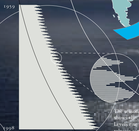
MONTHLY CO 2 CONCENTRATIONS MEASURED AT MAUNA LOA, HAWAII
