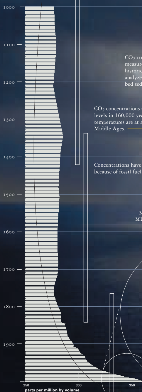
ATMOSPHERIC CONCENTRATIONS OF CARBON DIOXIDE (CO 2 )
