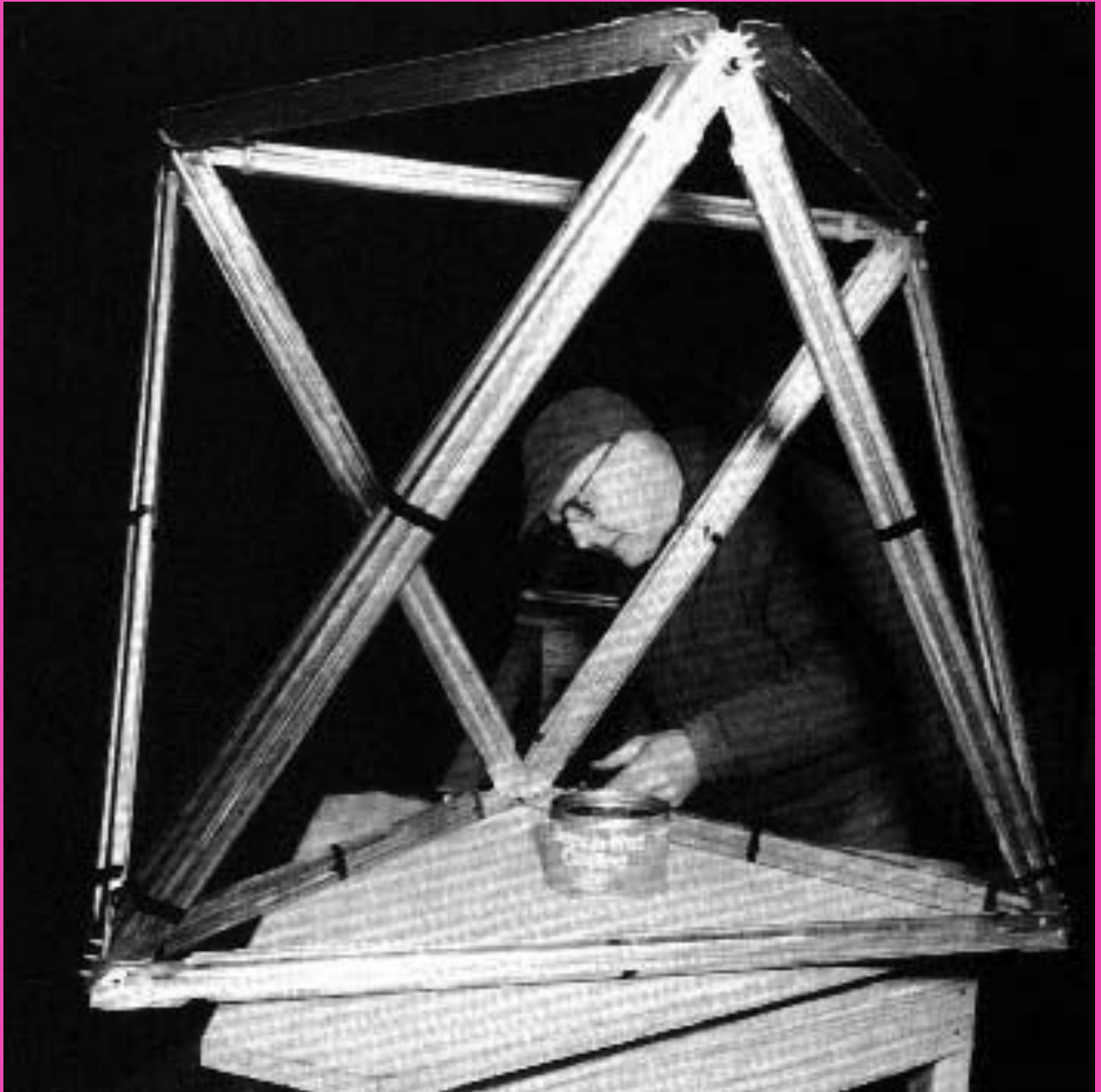
The octahedron-tetrahedron complex has been discovered and formulated within various contexts: chemistry, physics, mathematics and other. A construction system (the "octet truss") which makes use of this geometry was patented in the 1940's by R. Buckminster Fuller, USA. The system was used as a curved space frame for building the Ford Rotunda in Detroit.
