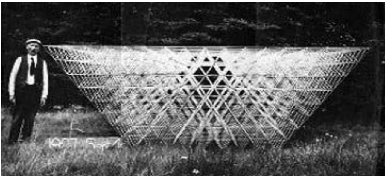
Alexander Graham Bell, in his search for lightweight structures for flight, discovered the octahedron-tetrahedron complex (the octet truss) in 1903, and used it for constructions such as kites, a windbreak and an observation tower.
